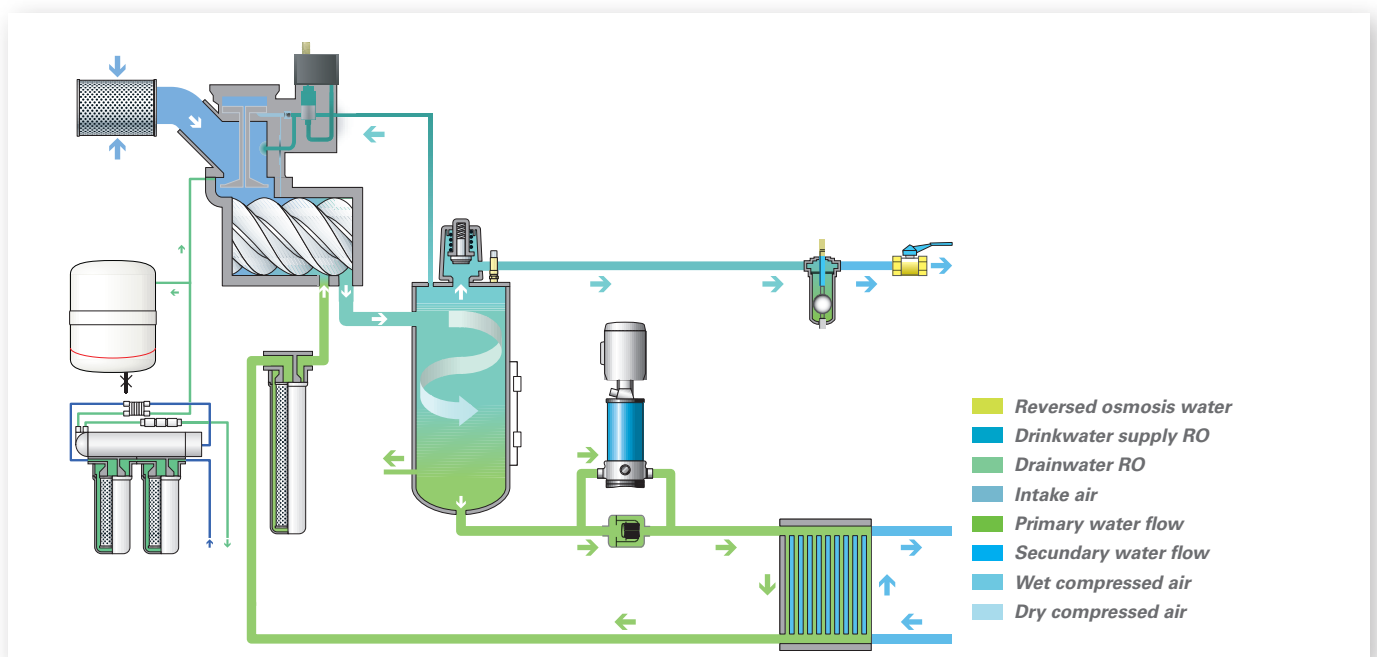
FLOW DIAGRAM AQ WATER-COOLED PACK
